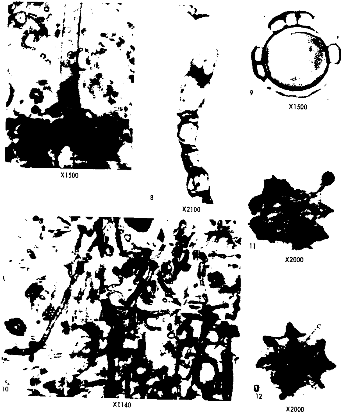
FIGURE 1.—Representative microfossils, three-dimensionally preserved in chert from the Gunfint iron-formation of the north shore of Lake Superior. This formation is of middle Precambrian age and has been dated by K^{40} - Ar^{40} as approximately 2 \times 10^9 years. All figures are from thin sections of the chert photographed in transmitted light. Published here for the first time (from Dr. E. S. Barghoorn).
