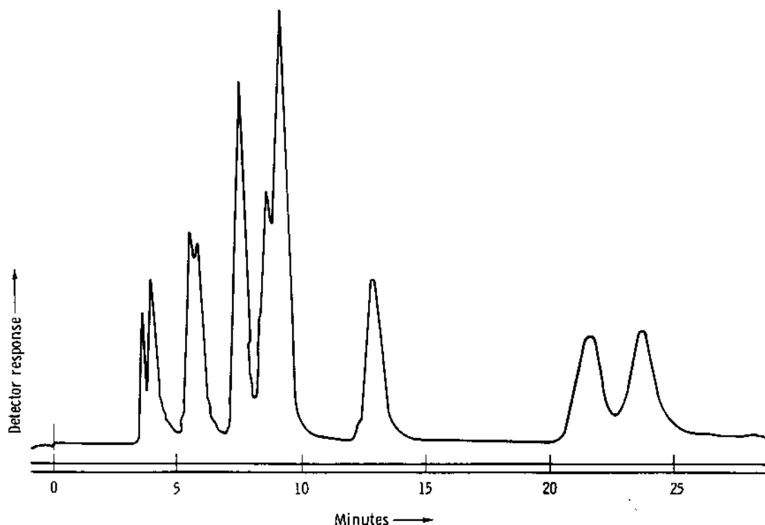
FIGURE 7.—Typical gas chromatogram. Zero is the time of injection. The time on the minutes scale, for each peak, is its retention time , and identifies the gas passing through the detector. The area under each peak is proportional to the amount of gas.
